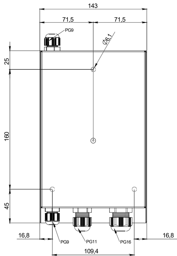
BOTTOM VIEW
